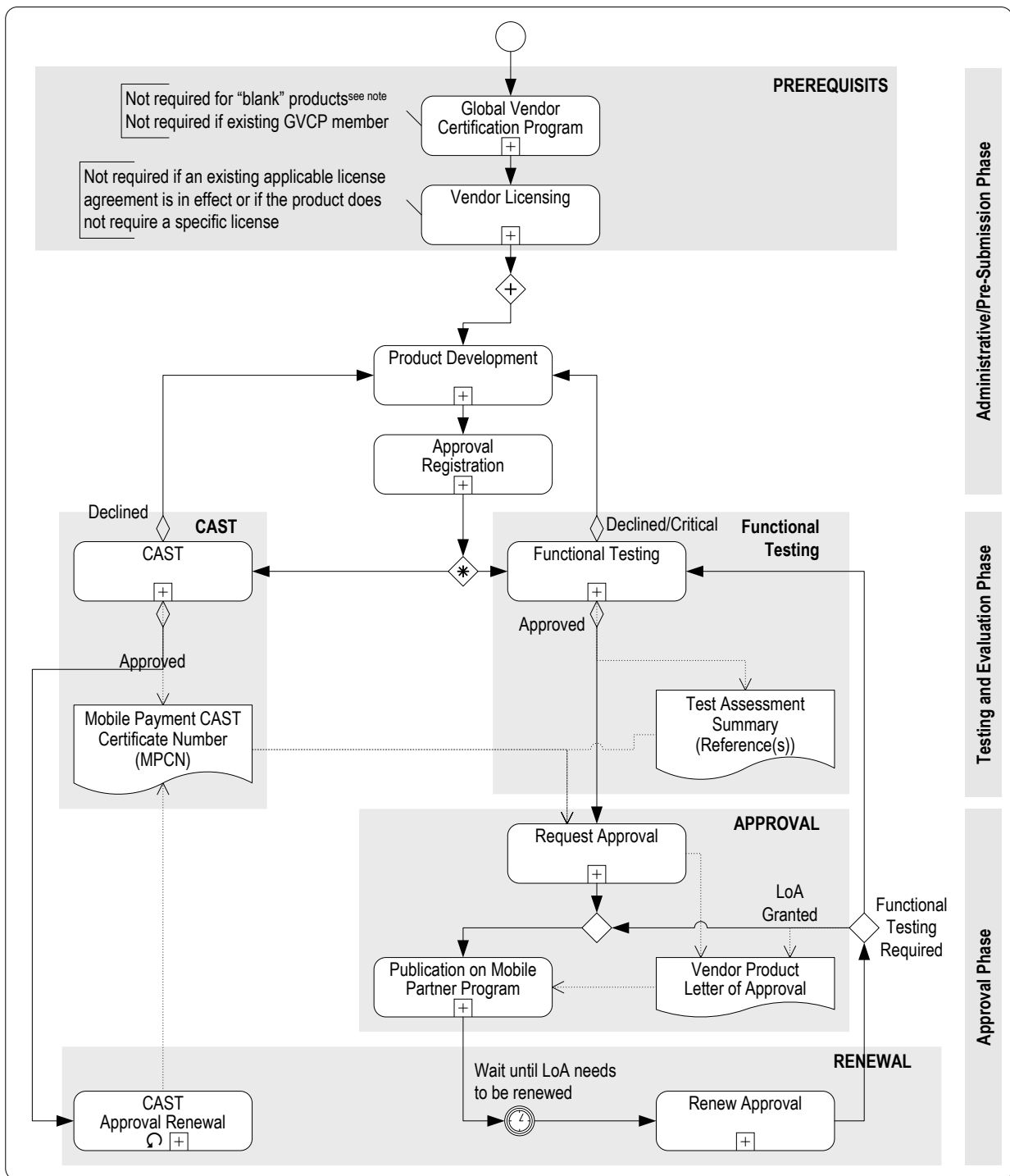
Figure 2-1 – M/Chip Mobile Secure Element Approval Process
